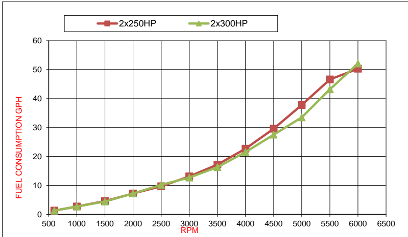
Fuel Consumption in Gallons per Hour
