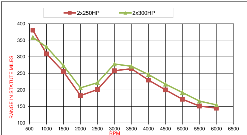
Range in Statute Miles
