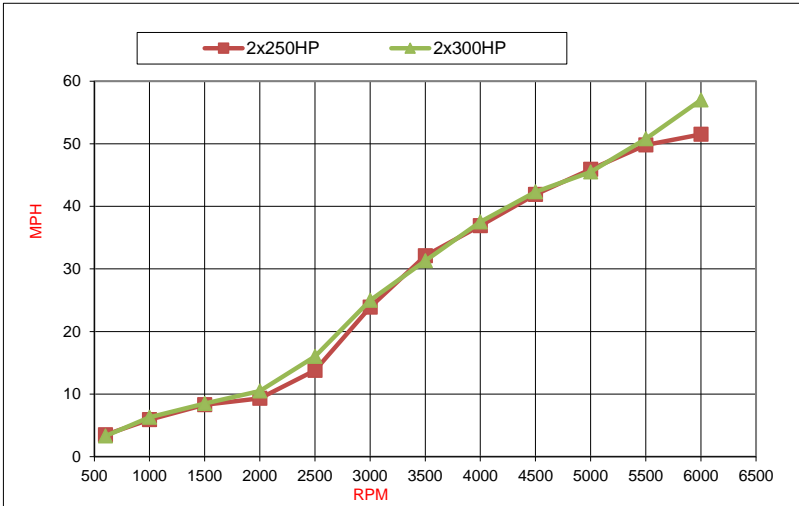
Speed in Miles per Hour
